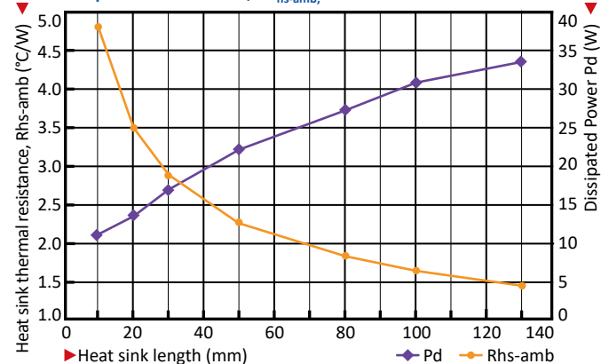
XSA-213 performance data at a heat sink to ambient temperature difference, \Delta T_{hs-amb} , of 50 °C
