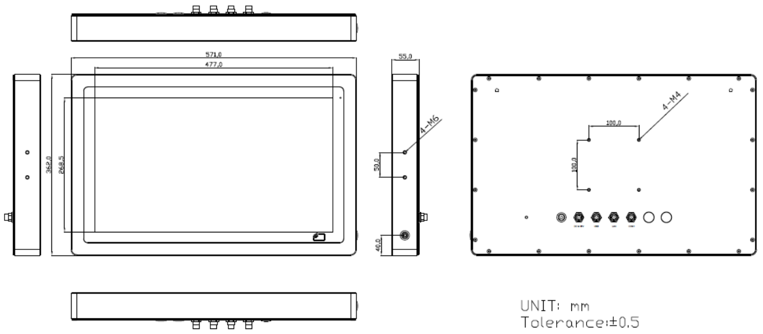
Figure 1.7: Dimensions of ViTAM-821P/R/G(H)
