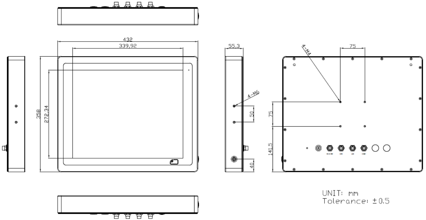
Figure 1.5: Dimensions of ViTAM-817P/R/G(H)
