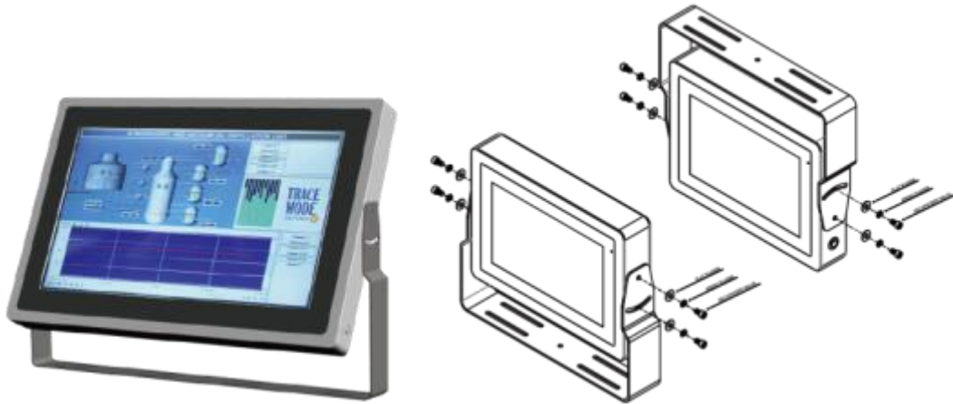
Figure 1.11: Yoke mounting of ViTAM-8XX Series
