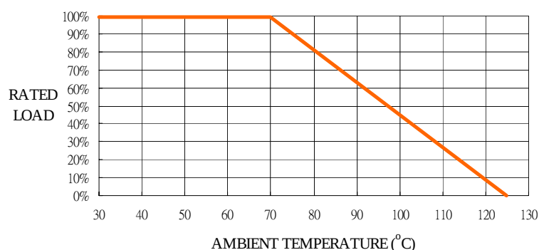
POWER DERATING CURVE
