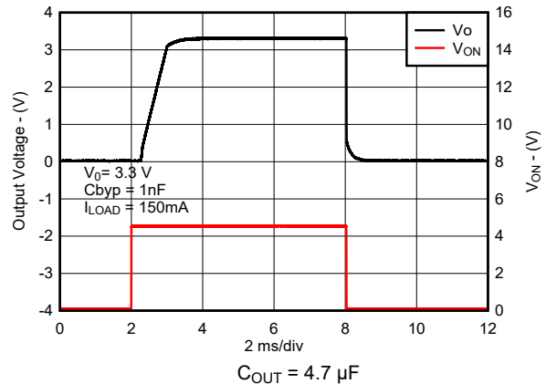
Figure 8-26. Turn-On Time for New Chip
