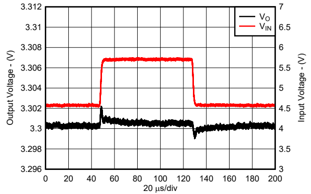
Figure 8-20. Line Transient Response for New Chip
