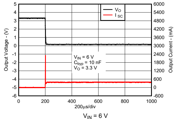
Figure 8-4. Short-Circuit Current for New Chip at V_{IN} = 6 V
