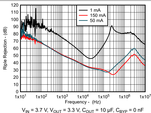
Figure 6-21. Ripple Rejection vs Frequency for New Chip
