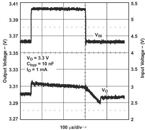
Figure 8-15. Line Transient Response for Legacy Chip
