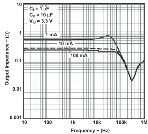
Figure 6-26. Output Impedance vs Frequency for Legacy Chip
