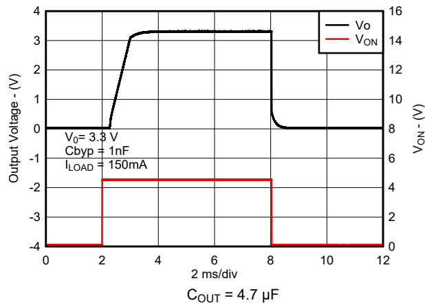
Figure 8-22. Turn-On Time for New Chip
