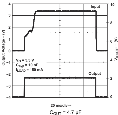
Figure 8-23. Turn-On Time
