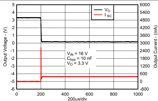
Figure 6-10. Short-Circuit Current vs Time for New Chip
