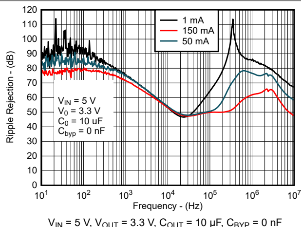
Figure 6-19. Ripple Rejection vs Frequency for New Chip
