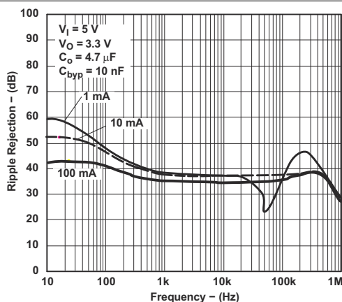
Figure 6-22. Ripple Rejection vs Frequency for Legacy Chip
