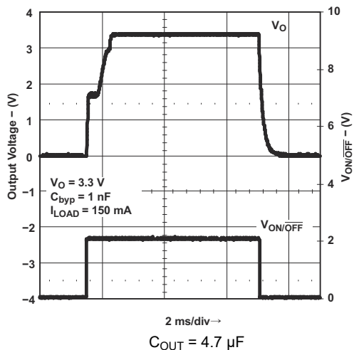
Figure 8-21. Turn-On Time for Legacy Chip
