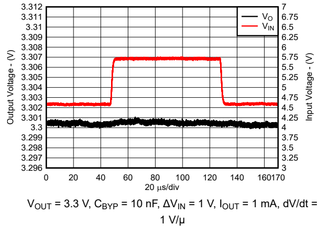
Figure 8-16. Line Transient Response for New Chip
