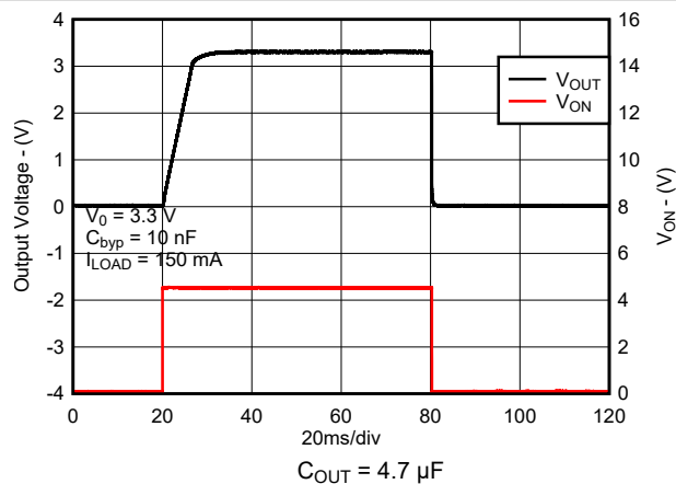
Figure 8-24. Turn-On Time for New Chip
