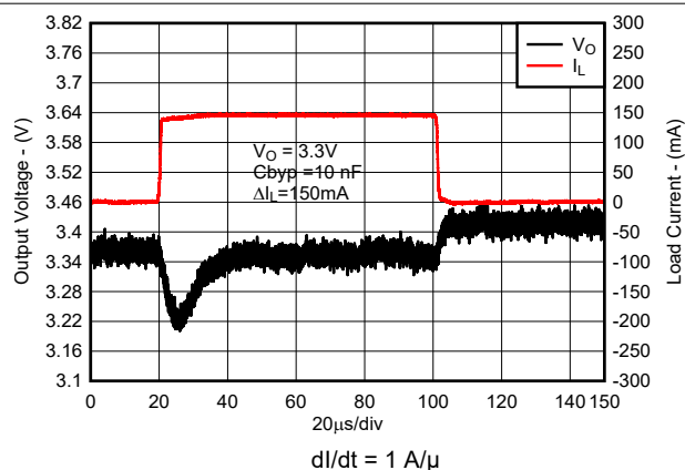
Figure 8-6. Load Transient for New Chip
