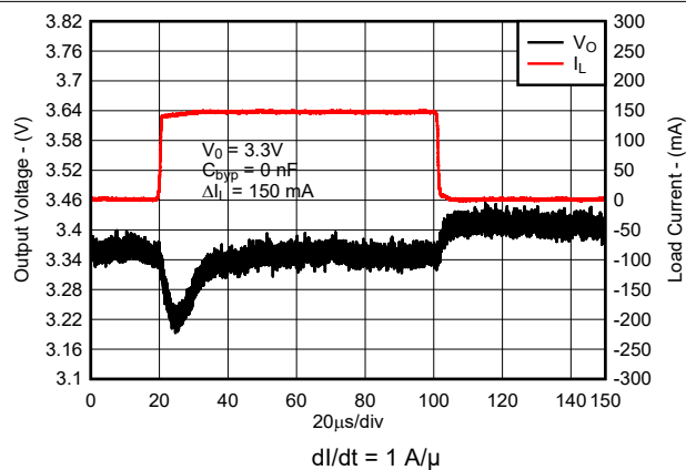
Figure 8-8. Load Transient Response for New Chip
