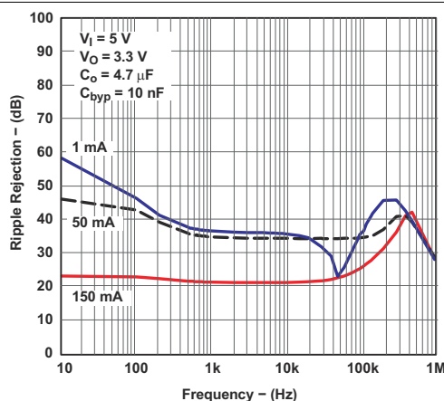
Figure 6-20. Ripple Rejection vs Frequency for Legacy Chip
