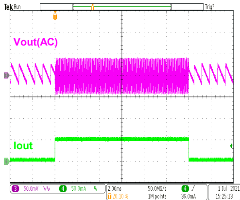
HT7722B Load Transient (1mA to 50mA)
