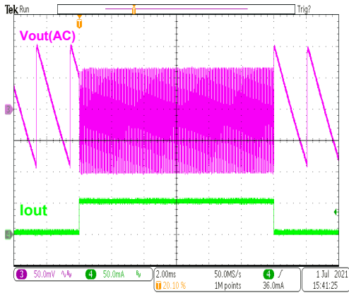
HT7750B Load Transient (1mA to 50mA)
