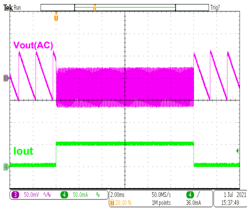
HT7737B Load Transient (1mA to 50mA)
