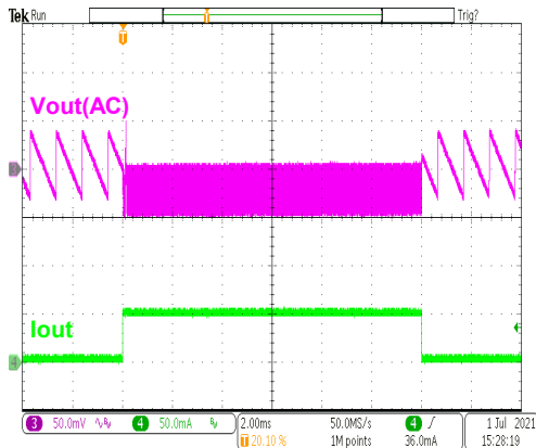
HT7727B Load Transient (1mA to 50mA)
