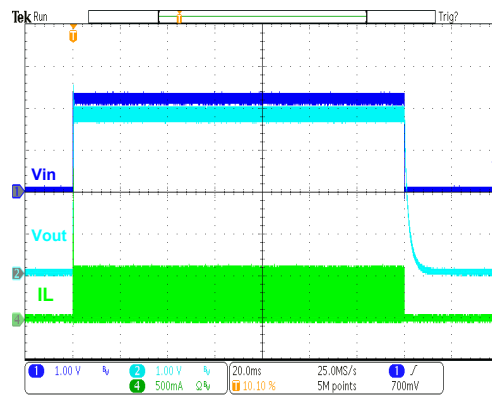
HT7737B Power On/Off ( V_{IN}=2.22V , I_{OUT}=50mA )
