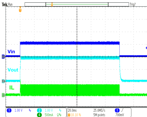
HT7718B Power On/Off ( V_{IN}=1.08V , I_{OUT}=50mA )
