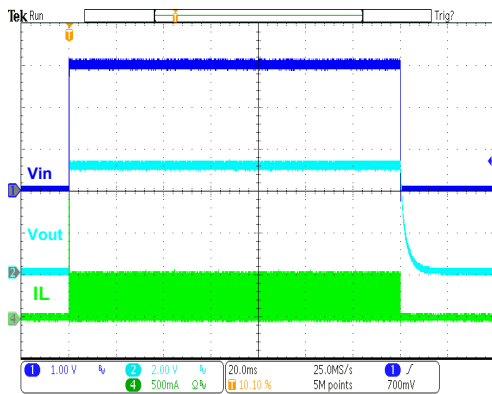
HT7750B Power On/Off ( V_{IN}=3V , I_{OUT}=50mA )
