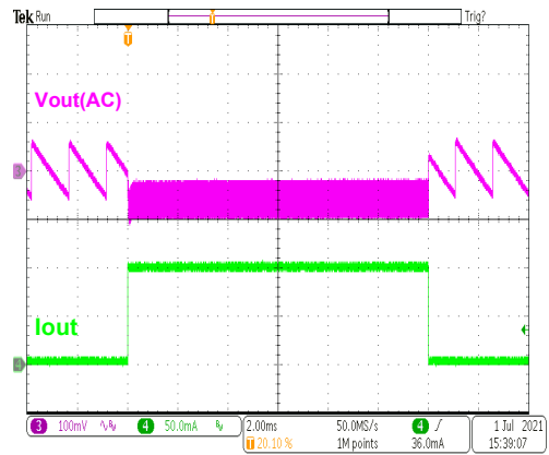
HT7737B Load Transient (1mA to 100mA)
