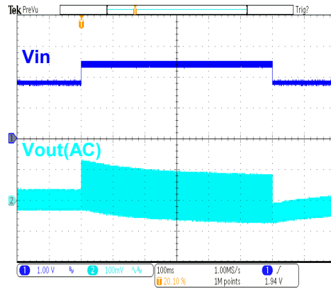
HT7730B Load Transient (1.8V~2.4V, I_{OUT}=50mA )
