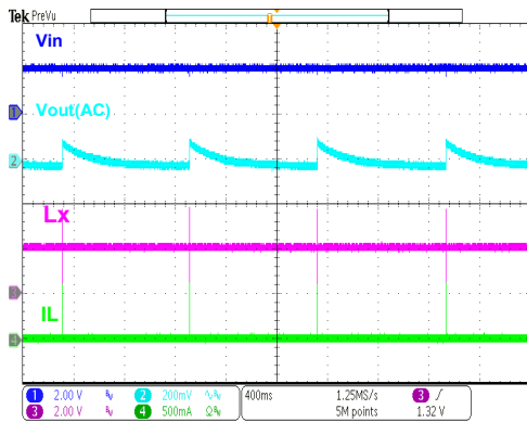
HT7733B Operation ( I_{out}=0mA )
