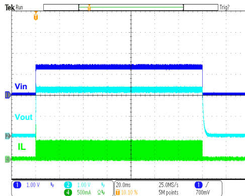
HT7722B Power On/Off ( V_{IN}=1.32V , I_{OUT}=50mA )
