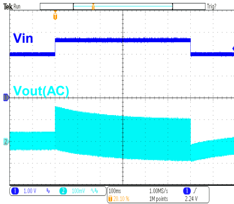
HT7733B Load Transient (1.98V~2.64V, I_{OUT}=50mA )
