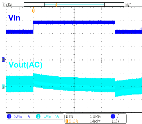
HT7718B Load Transient (1.08V~1.44V, I_{OUT}=50mA )
