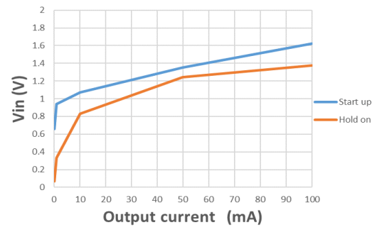
HT7750B Startup/Hold-on Voltage
