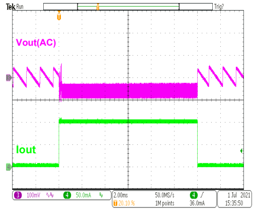
HT7733B Load Transient (1mA to 100mA)
