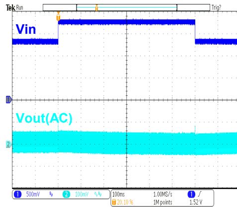
HT7722B Load Transient (1.32V~1.76V, I_{OUT}=50mA )
