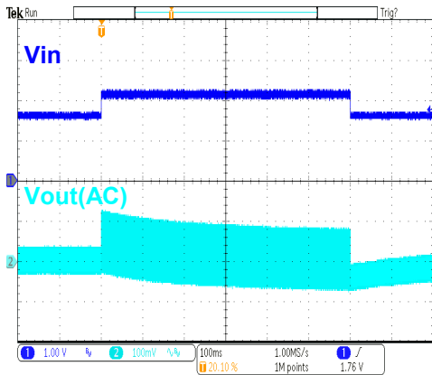
HT7727B Load Transient (1.62V~2.16V, I_{OUT}=50mA )
