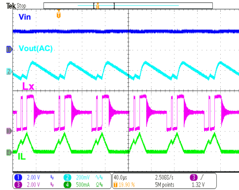
HT7730B Operation ( I_{out}=50mA )
