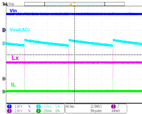
HT7722B Operation ( I_{out}=0mA )
