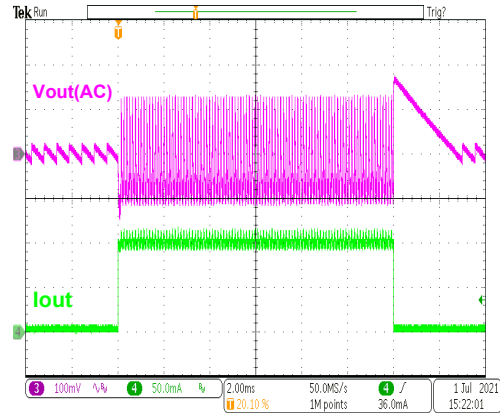
HT7718B Load Transient (1mA to 100mA)
