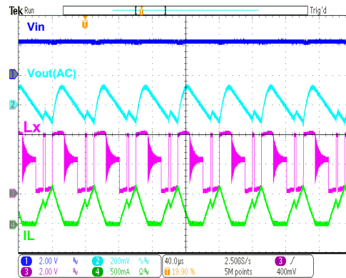
HT7737B Operation ( I_{out}=50mA )
