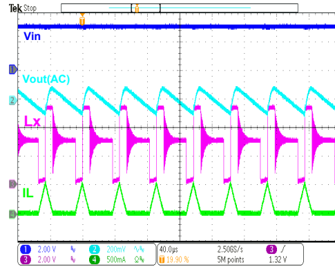
HT7750B Operation ( I_{OUT}=50mA )
