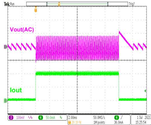
HT7722B Load Transient (1mA to 100mA)
