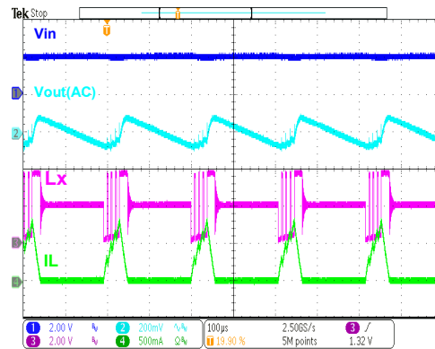
HT7733B Operation ( I_{out}=50mA )
