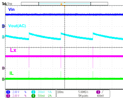
HT7737B Operation ( I_{out}=0mA )
