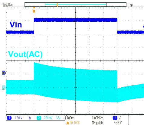
HT7750B Load Transient (3V~4V, I_{OUT}=50mA )
