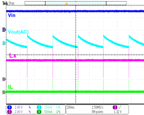
HT7750B Operation ( I_{OUT}=0mA )
