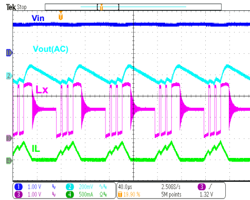
HT7722B Operation ( I_{out}=50mA )
