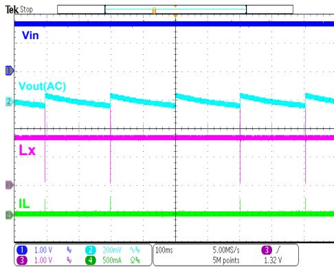
HT7727B Operation ( I_{out}=0mA )
