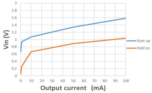
HT7737B Startup/Hold-on Voltage
