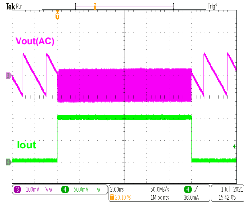
HT7750B Load Transient (1mA to 100mA)
