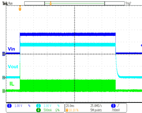
HT7727B Power On/Off ( V_{IN}=1.62V , I_{OUT}=50mA )
