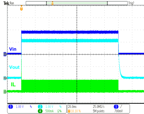
HT7733B Power On/Off ( V_{IN}=1.8V , I_{OUT}=50mA )
