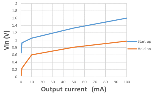
HT7733B Startup/Hold-on Voltage
