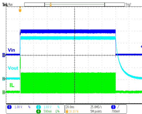
HT7733B Power On/Off ( V_{IN}=1.98V , I_{OUT}=50mA )
