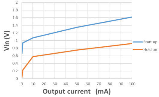
HT7730B Startup/Hold-on Voltage
