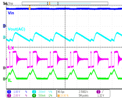
HT7727B Operation ( I_{out}=50mA )
