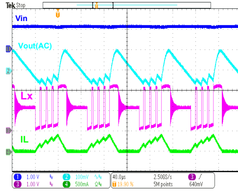
HT7718B Operation ( I_{out}=50mA )
