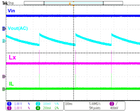
HT7718B Operation ( I_{out}=0mA )
