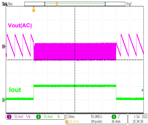
HT7733B Load Transient (1mA to 50mA)
