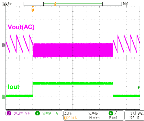
HT7730B Load Transient (1mA to 50mA)
