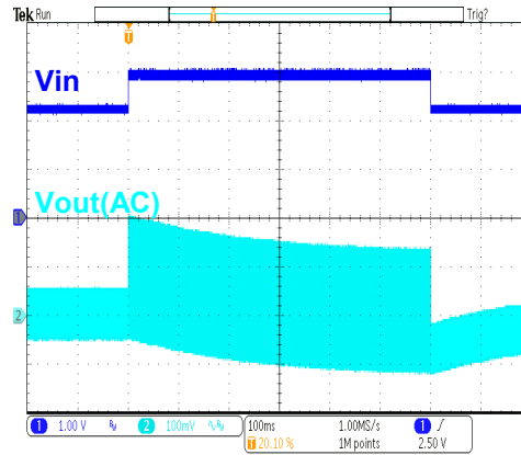
HT7737B Load Transient (2.22V~2.96V, I_{OUT}=50mA )
