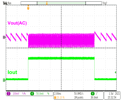
HT7730B Load Transient (1mA to 100mA)
