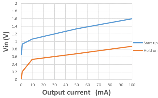
HT7727B Startup/Hold-on Voltage
