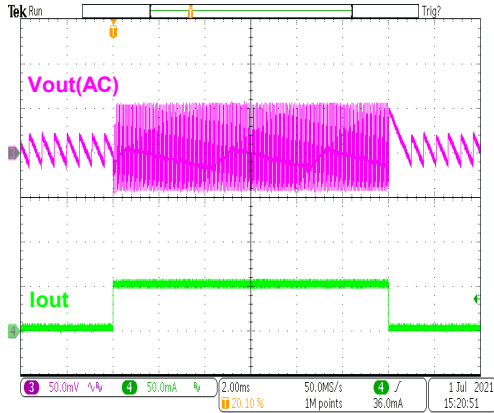
HT7718B Load Transient (1mA to 50mA)
