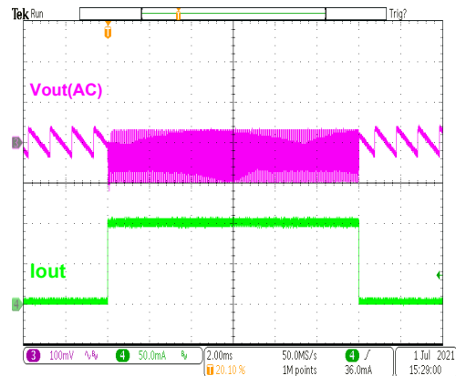
HT7727B Load Transient (1mA to 100mA)
