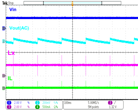
HT7730B Operation ( I_{out}=0mA )
