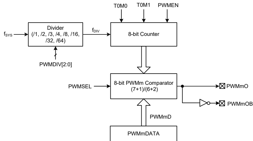
PWM Mode Block Diagram
