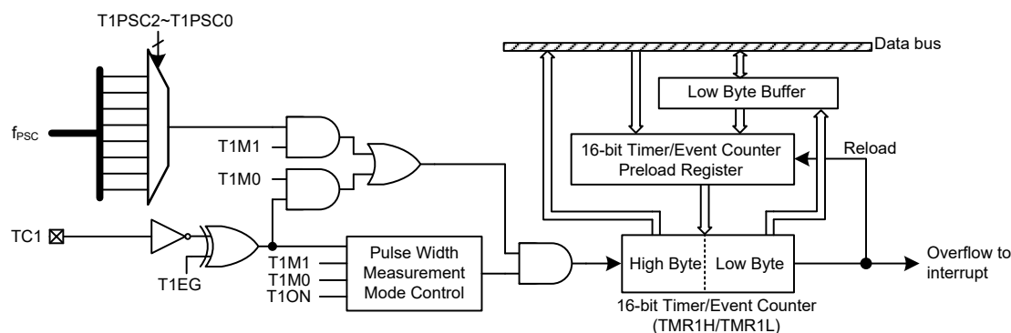
16-bit Timer/Event Counter Structure
