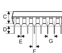
Fig1. 1/2 Lead Packages
