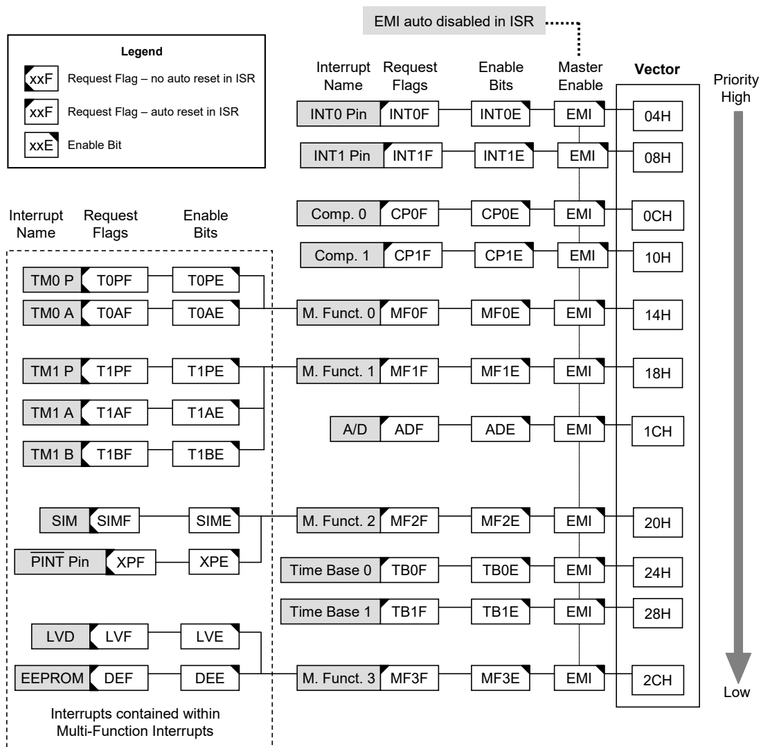
Interrupt Structure – HT66F20-1/HT66F30-1
