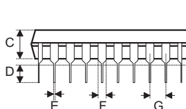
Fig2. 1/2 Lead Packages
