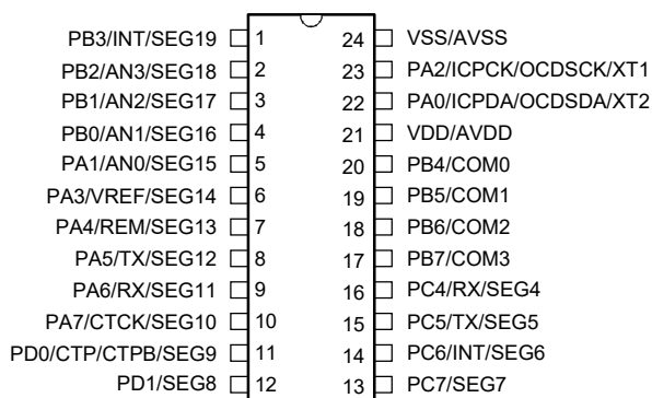
HT67F2432/HT67V2432 24 SSOP-A
