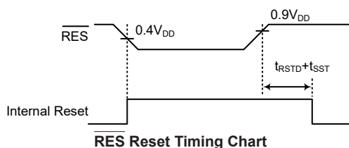
RES Reset Timing Chart
