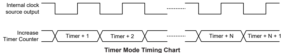
Timer Mode Timing Chart
