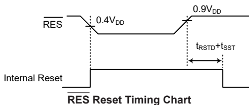
RES Reset Timing Chart
