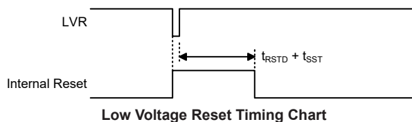
Low Voltage Reset Timing Chart
