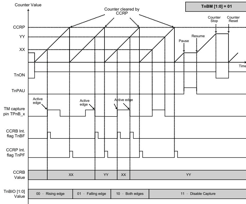
ETM CCRB Capture Input Mode
