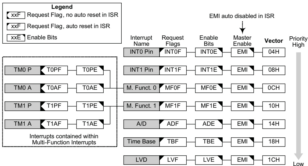
Interrupt Structure – HT66F14
