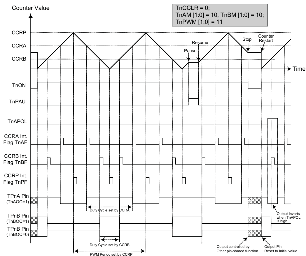
ETM PWM Mode -- Centre Aligned
