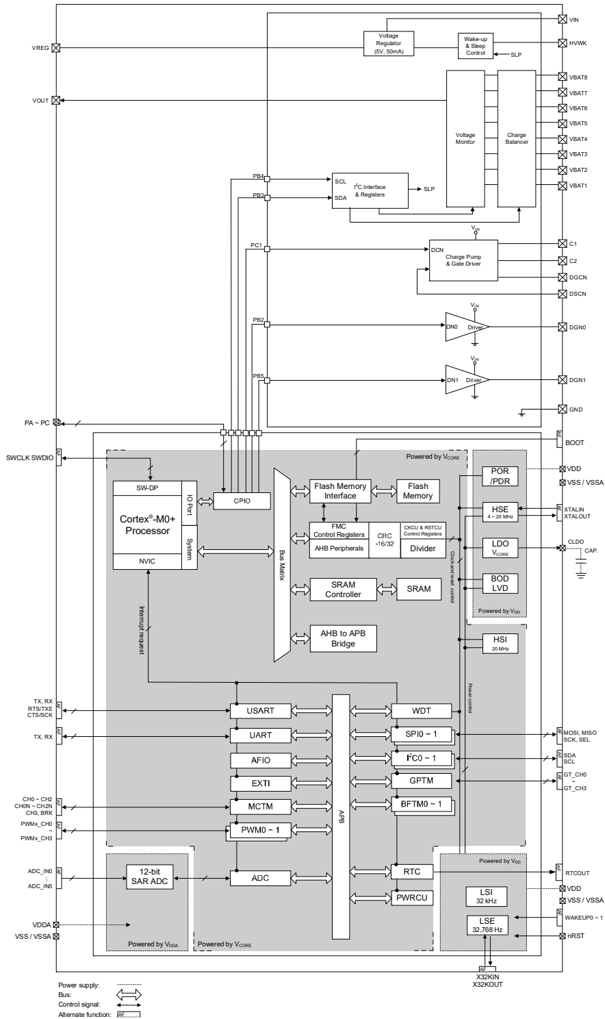
Figure 1. Block Diagram
