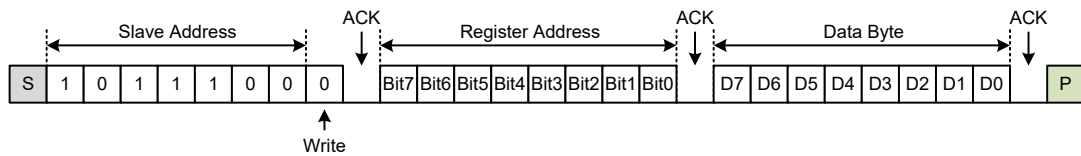
Figure 9. Write Operation Format
