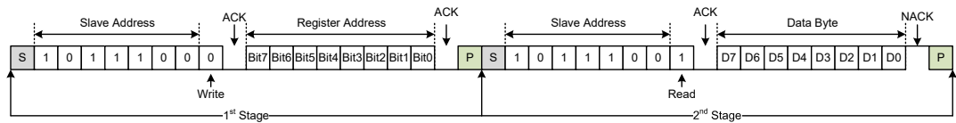
Figure 10. Read Sequence Format
