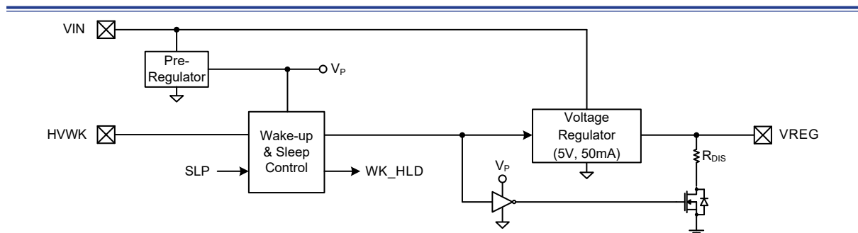
Figure 14. Wake up from Sleep Mode Functional Block Diagram
