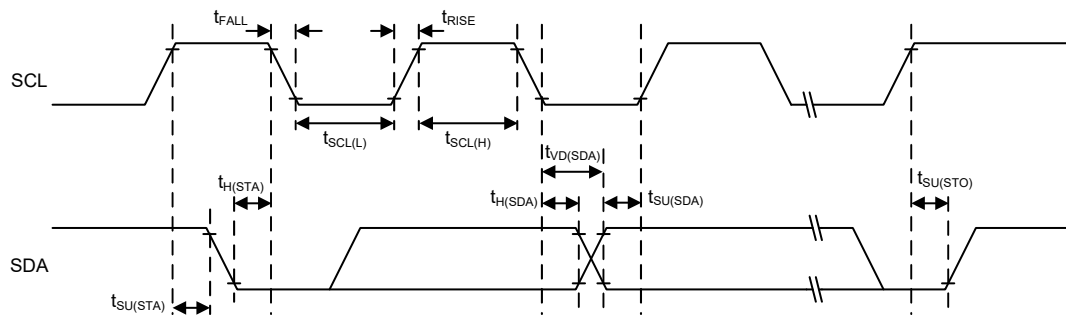
Figure 29. I 2 C Timing Diagrams
