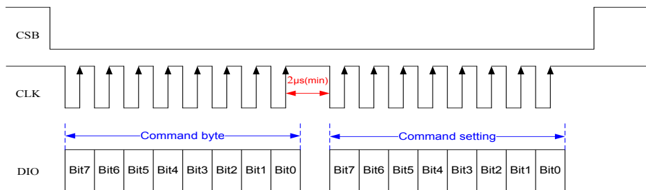
SPI Compound Command Type Write Operation
