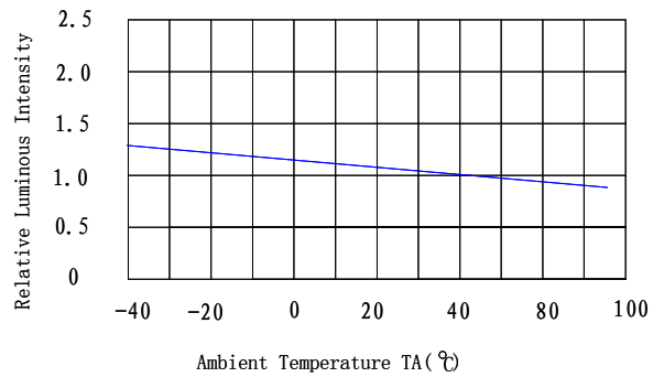
Relative Luminous Intensity vs Ambient Temperature
