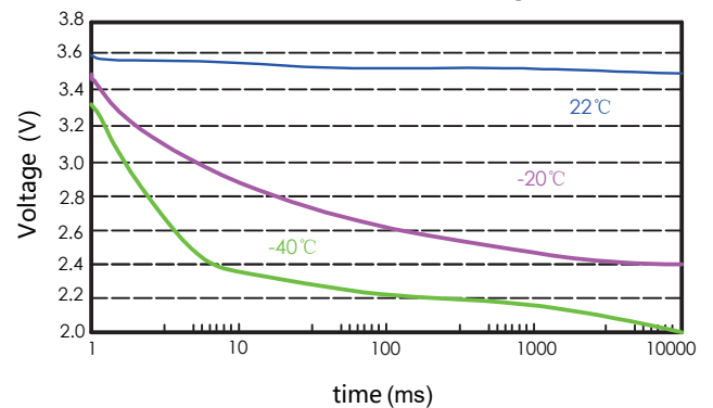
2. UPC1550 1000mA Discharge Curve
