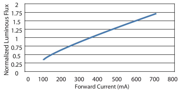
Figure 12. Relative luminous flux vs. forward current for Cool White, True Green, Blue, Cyan, Dental Blue and Royal Blue ,at T_j = 25^\circ\text{C} .
