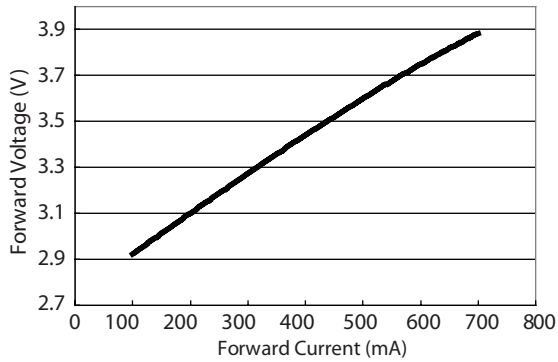
Figure 9. Forward voltage vs. forward current for White, Blue, Dental Blue and Royal Blue ,at T_j = 25^\circ\text{C} .
