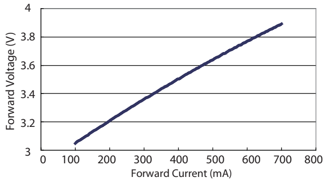
Figure 10. Forward voltage vs. forward current for True Green and Cyan ,at T_j = 25^\circ\text{C} .
