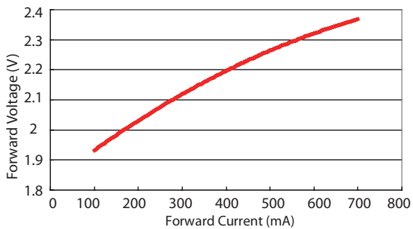
Figure 11. Forward voltage vs. forward current for Red and Amber ,at T_j = 25^\circ\text{C} .
