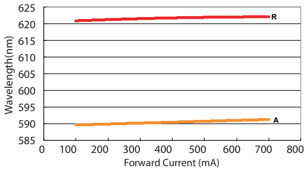
Figure 15. Wavelength length vs. forward current for Red and Amber, at T_j = 25^\circ\text{C} .
