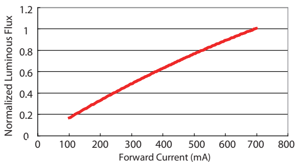
Figure 13. Relative luminous flux vs. forward current for Red and Amber ,at T_j = 25^\circ\text{C} .
