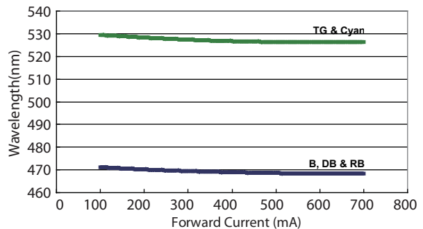
Figure 14. Wavelength length vs. forward current for True Green, Blue, Cyan, Royal Blue and Dental Blue ,at T_j = 25^\circ\text{C} .
