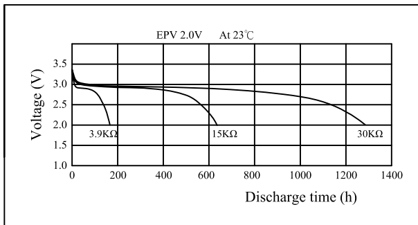
Discharge characteristics
