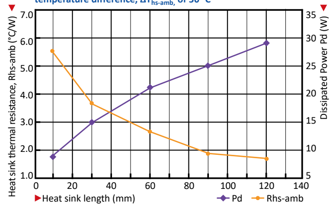
CoolStar® 67 performance data at a heat sink to ambient temperature difference, ΔT hs-amb , of 50 °C
