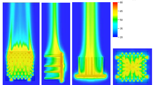
CoolBlock® thermal simulations results CFD
