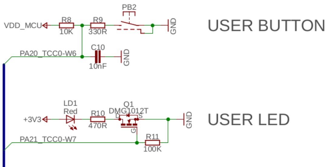
Figure 11 – ATSAM21 Pushbuttons and Leds
