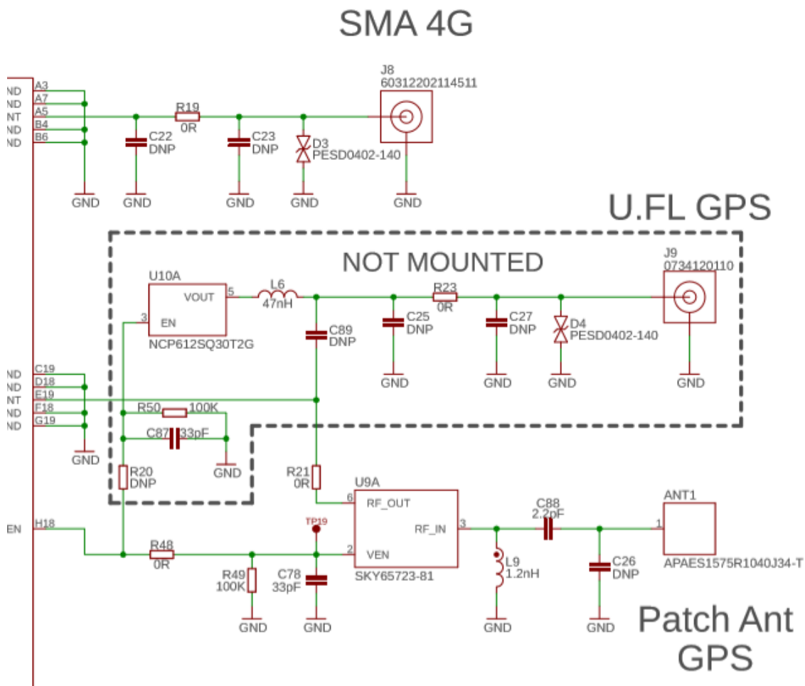
Figure 8 – Antennas
