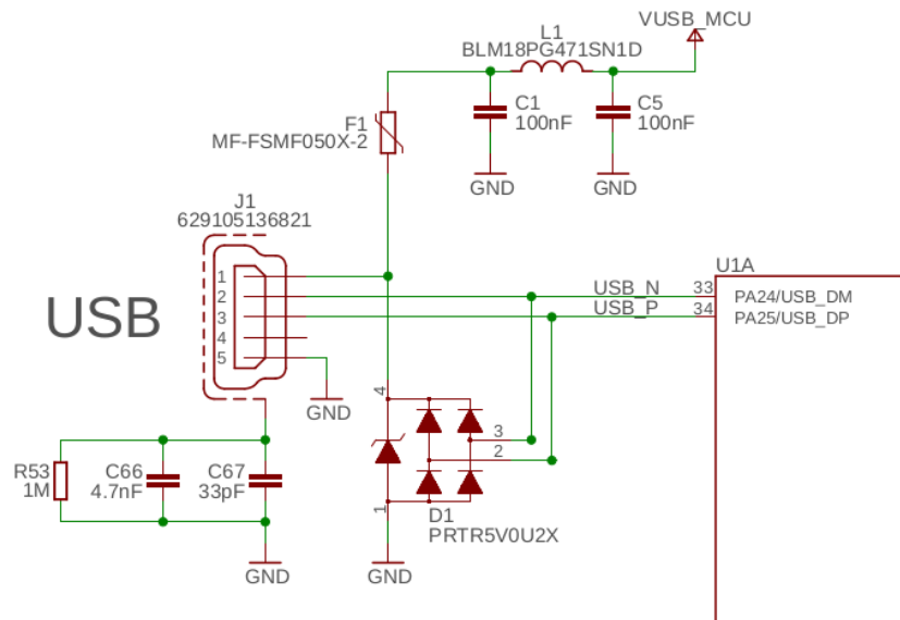
Figure 4 – ATSAMR21 Native USB
