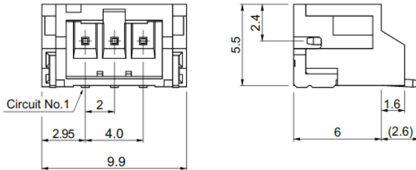
Figure 15 - Battery Connector
