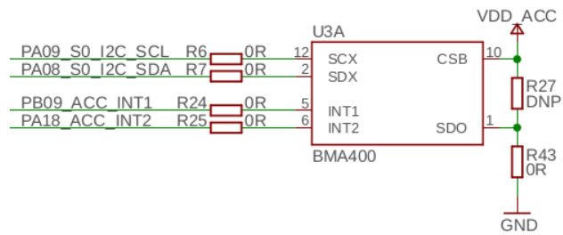
Figure 10 – BMA400 Accelerometer
