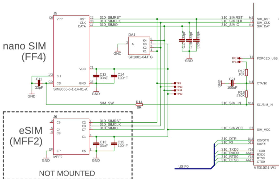
Figure 7 - SIM Sockets
