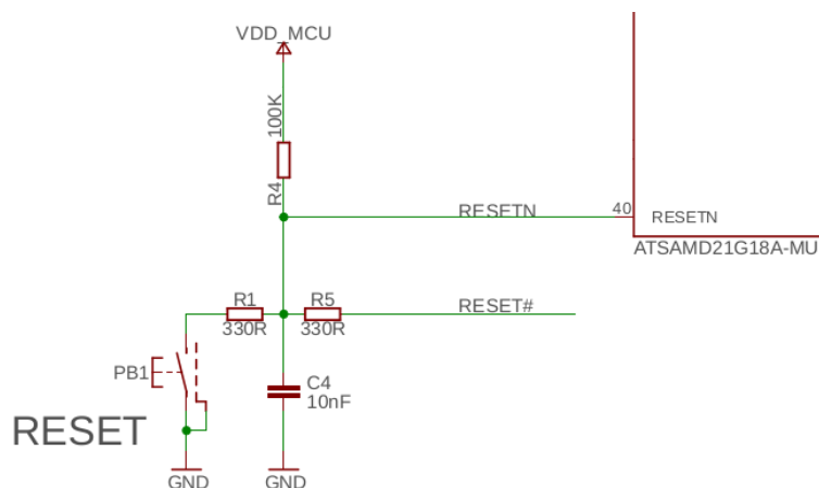
Figure 13 – RESET button
