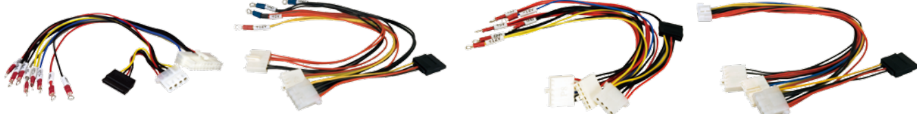
CB-716P8P9 CB-855P8P9 CB-870P8P9
