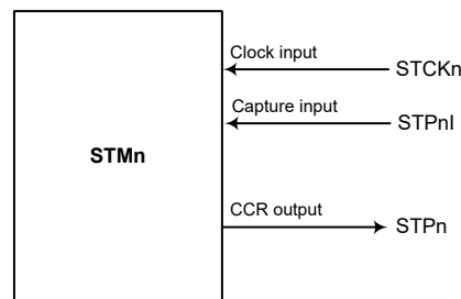
STMn Function Pin Block Diagram (n=0~1)
