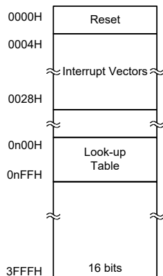
Program Memory Structure
