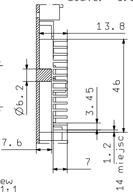
Section view D-D Scale: 1:1
